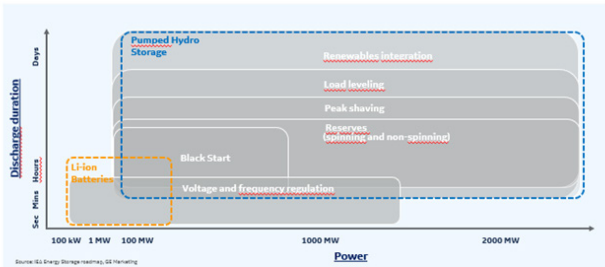
Figure 8. Contrast of PSH and Lithium-ion batteries with respect to size, storage duration and grid support services.
