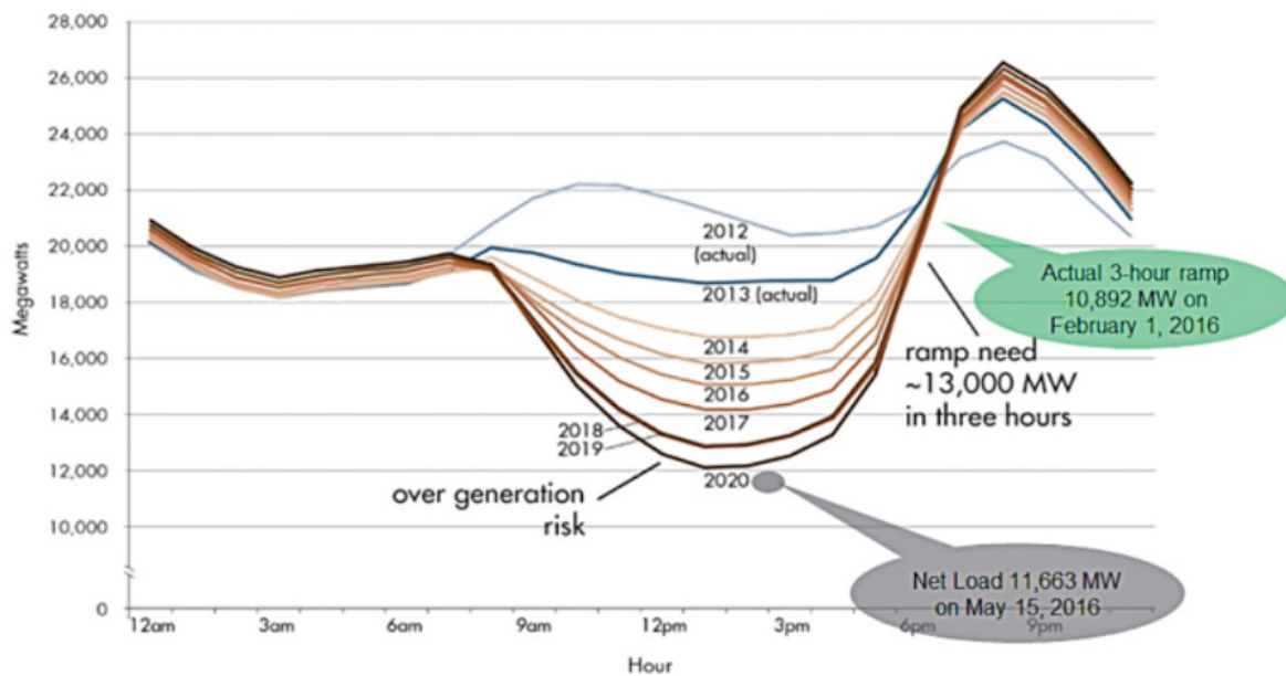
Figure 6. CAISO duck curve graphic illustrating potential daily future scenarios of net load covers.
